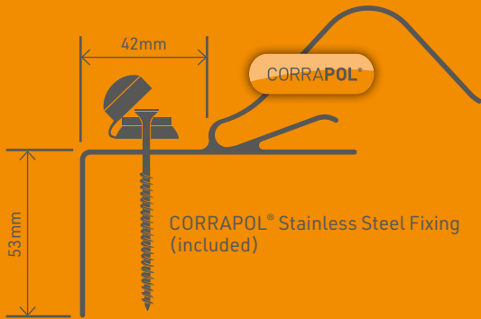
a CORRAPOL® Rock n' Lock Gable Flashing
