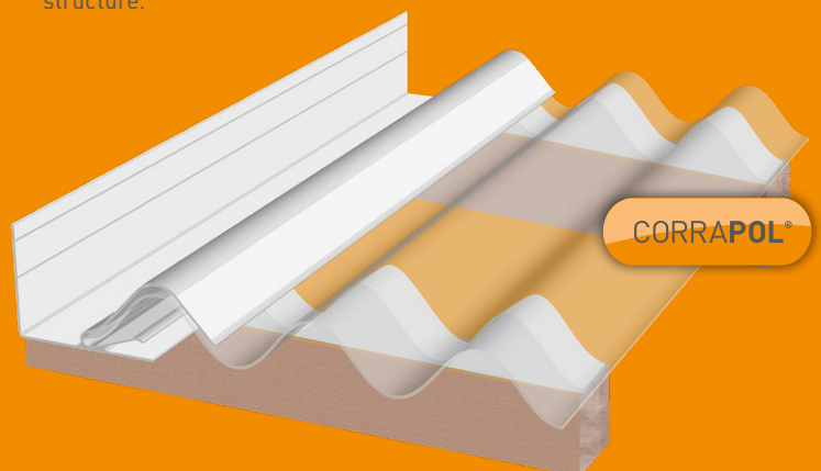
c Lock the CORRAPOL® Rock n' Lock Wall Flashing into place giving a waterproof and visually pleasing finish to the wall edge of your roof structure.
