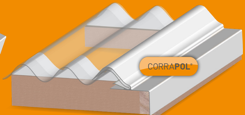
c Straighten the CORRAPOL® Rock n' Lock Gable Flashing into place giving a waterproof and visually pleasing finish to the edge of your roof structure.
