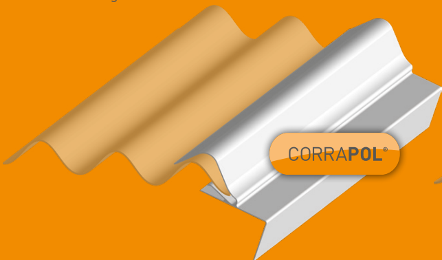
b Tilt the CORRAPOL® Rock n' Lock Gable Flashing to the side and fit the first corrugated sheet peak into the flashing.
