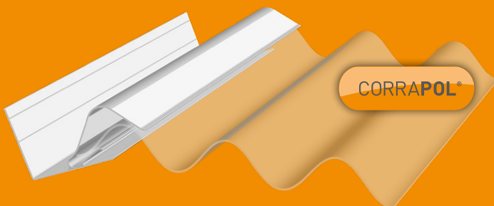
b Tilt the CORRAPOL® Rock n' Lock Wall Flashing to the side and fit the first corrugated sheet peak into the flashing.
