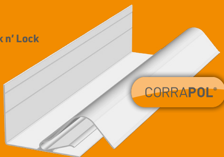
b Tilt the CORRAPOL® Rock n' Lock Wall Flashing to the side and fit the first corrugated sheet peak into the flashing.
