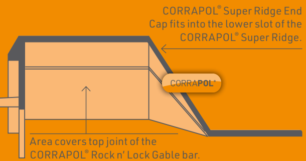
CROSS SECTION OF CORRAPOL® SUPER RIDGE END CAP
