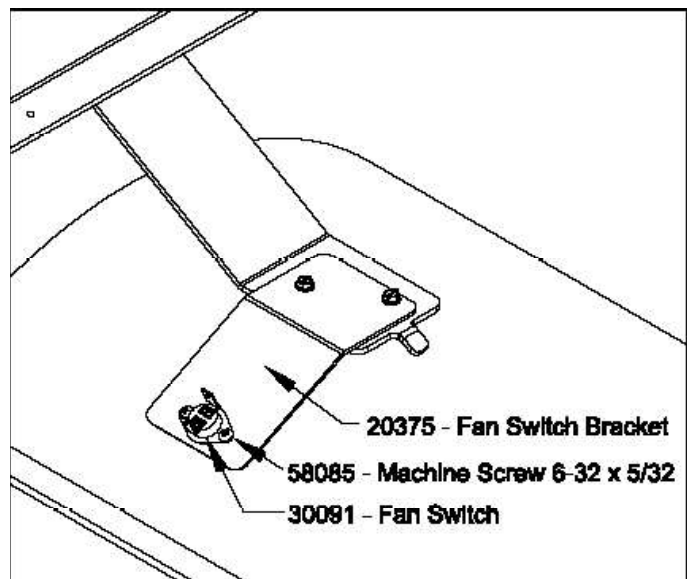
Figure 2: Install New Fan Switch (30091)
