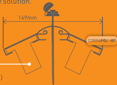
CORRAPOL®-BT Super Ridge Gasket (included)
