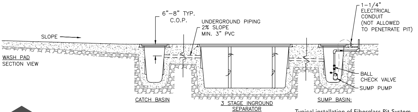
Typical installation of Fiberglass Pit System
